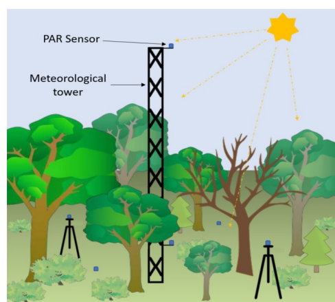
Figure 1.5.2 Photosynthetic photon flux density (PPFD) sensors should be arranged above the canopy ( n = 1 ), between the canopy and sub-canopy ( n varies depending on plot size/heterogeneity), and on the ground surface ( n varies depending on plot size and heterogeneity; tree clip-art made available by ian.umces.edu/imagelibrary ).
